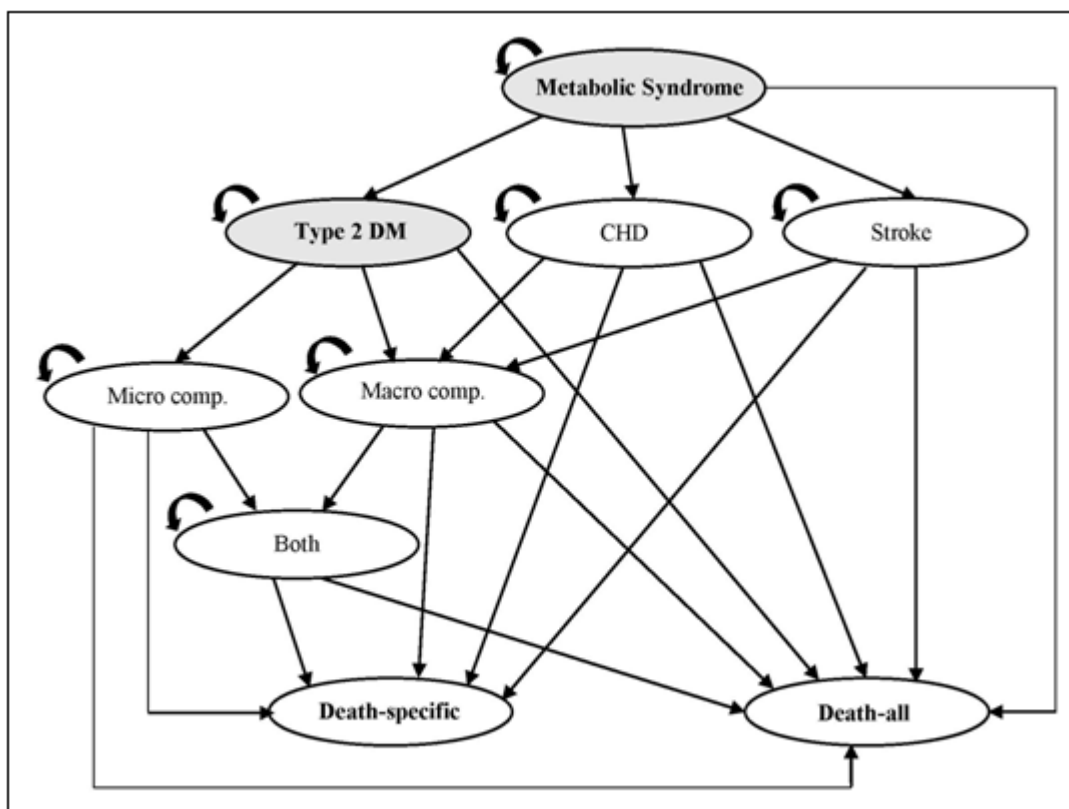
Figure 1. Markov model
